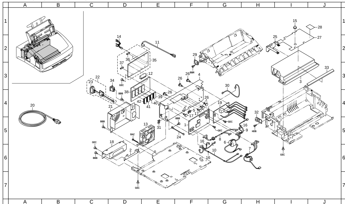
FIG. 7 ELECTRICAL COMPONENTS
