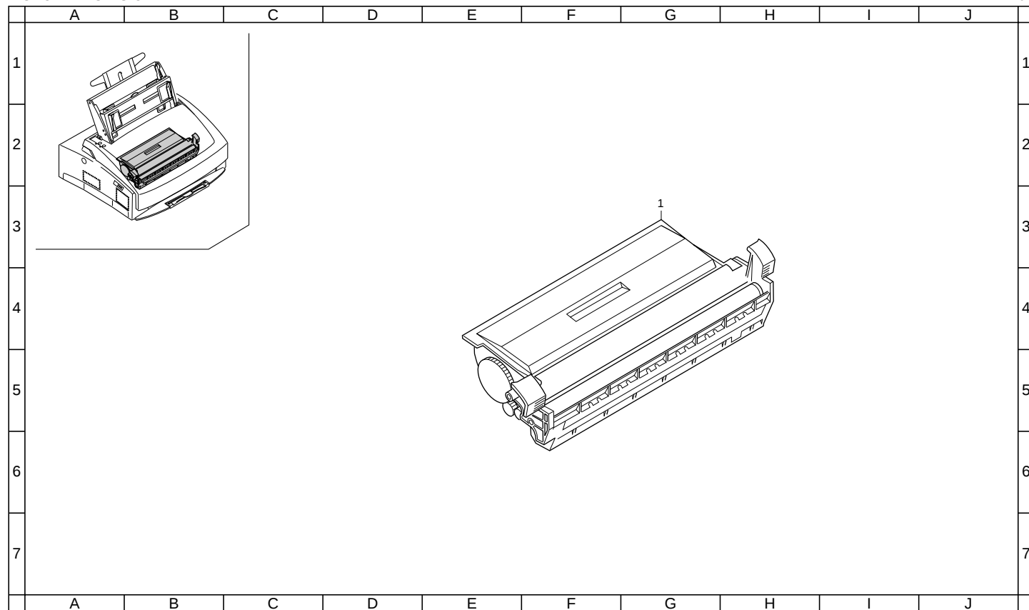
FIG. 8 IMAGING UNIT
