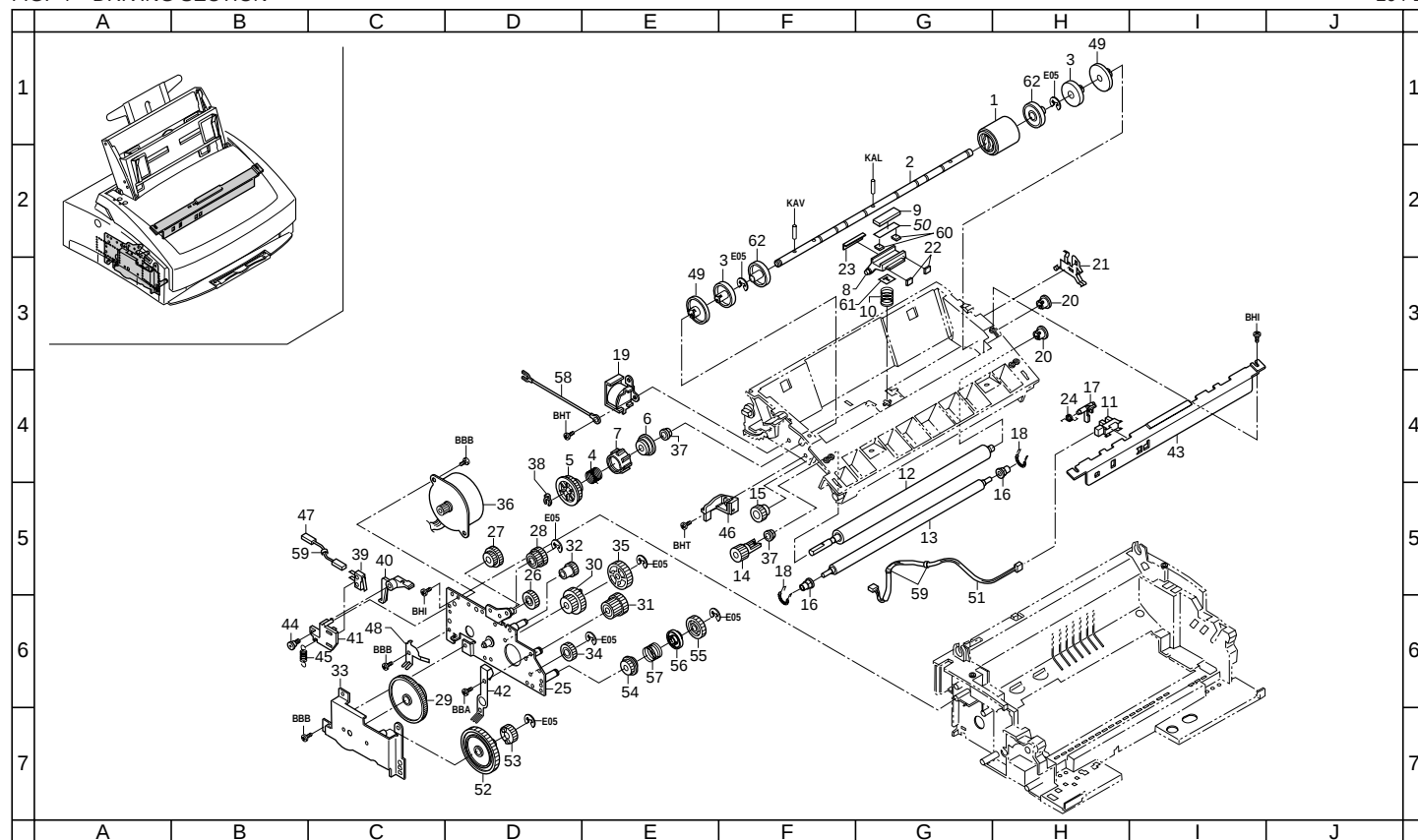
FIG. 4 DRIVING SECTION
